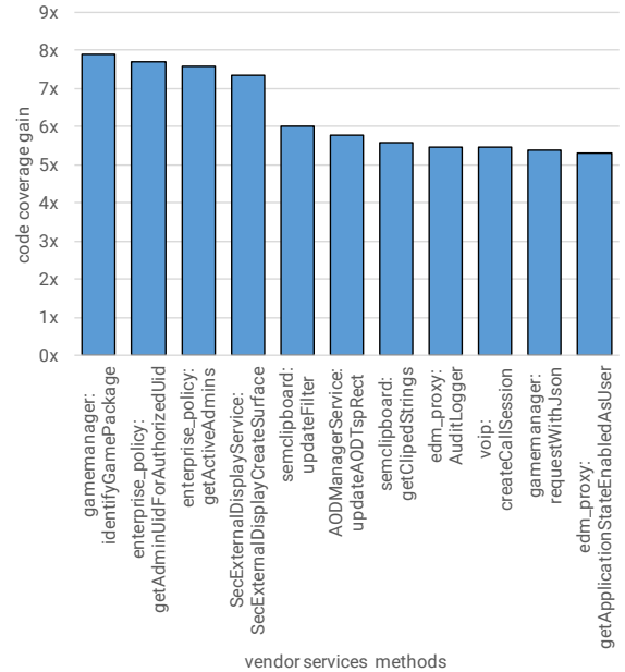
Fig. 6. Code Coverage Gain of Chizpurple per Method.
