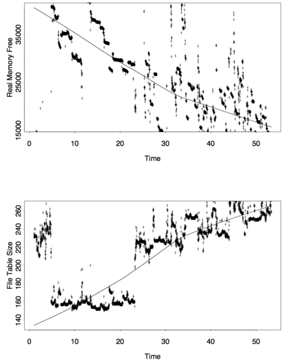
Fig. 1. Resource consumption measurements (free memory and file table size) from a SunOS workstation, and non-parametric regression smoothing to visualize trends [12].
