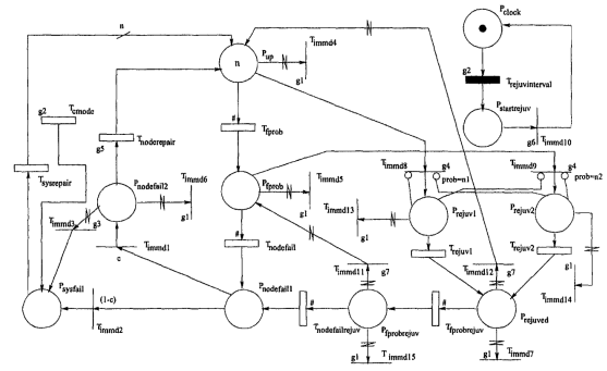
Fig. 3. Cluster system adopting time-based rejuvenation [25].
